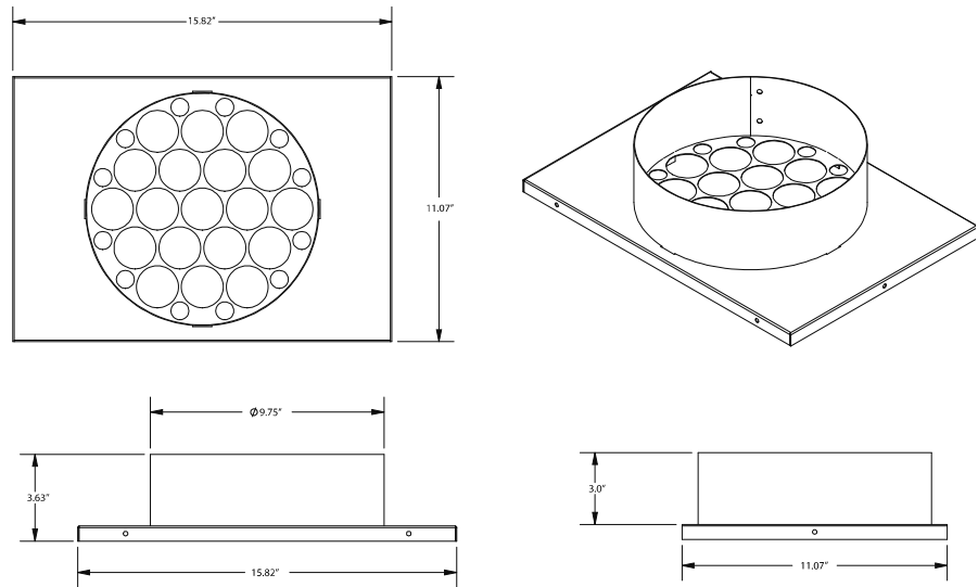
Fig. 1 – Square-to-Round Dimensional Detail
